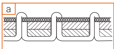
11-rasm. Mashina chokidagi kamchiliklar va tekis baxyaqator:
