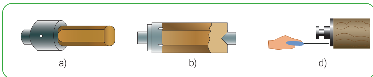
25-rasm. Tokarlik stanogida zagotovkalarni o'rnatish usullari: a) patronga o'rnatish; b) planshayba o'rnatish; d) planshaybaga o'rnatish.
