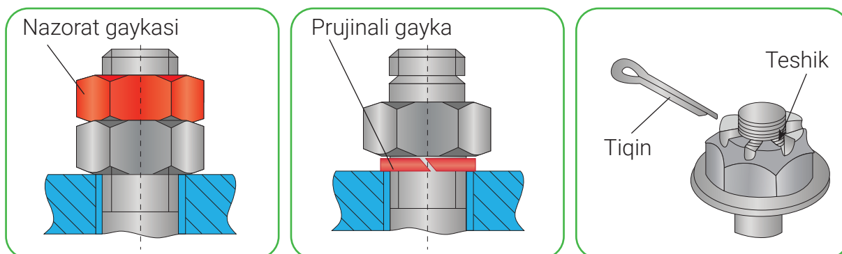
74-rasm. Rezbaning aylanish harakati to'xtatib qo'yiladigan rezballi birikmalar
