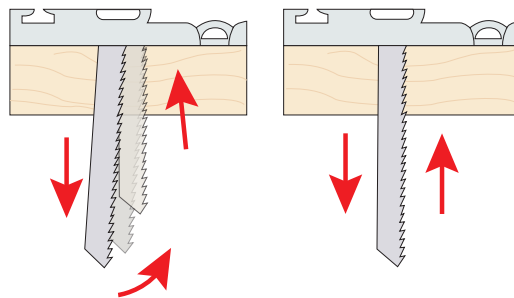
39-rasm. Lobzik polotnosining harakatlari
